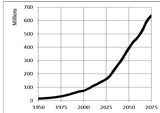
Fig. 12b. Increase of global number of elderly people (aged 80 years+), 1950–2015, with the UN medium forecast till 2075
